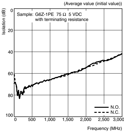
High-frequency Characteristics at 75 Ω (Isolation) (See notes 1 and 2.)
