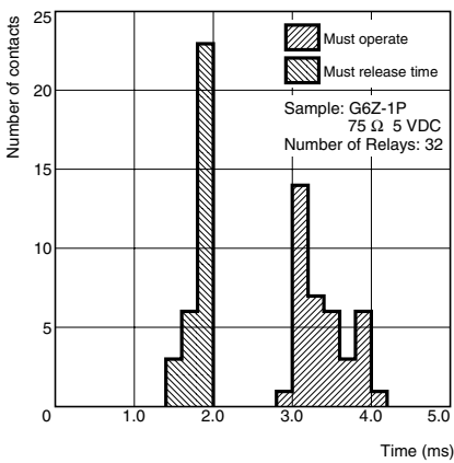
Must Operate and Must Release Time Distribution (See note 1.)
