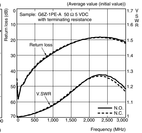
High-frequency Characteristics at 50 Ω (Return Loss, V.SWR) (See notes 1 and 2.)
