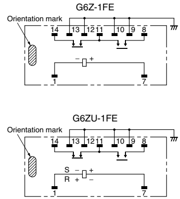
Terminal Arrangement/Internal Connections (Top View)
