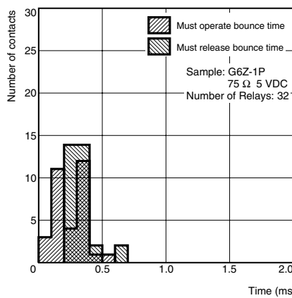
Must Operate and Must Release Bounce Time Distribution (See note 1.)
