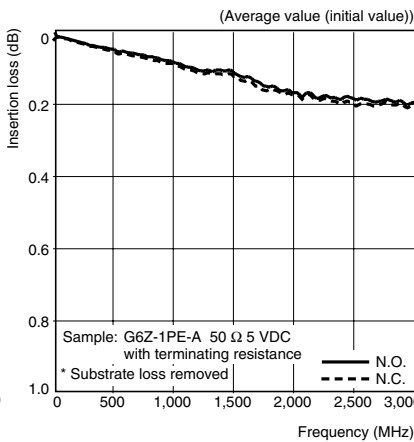
High-frequency Characteristics at 50 Ω (Insertion Loss) (See notes 1 and 2.)
