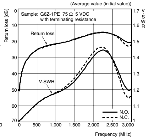
High-frequency Characteristics at 75 Ω (Return Loss, V.SWR) (See notes 1 and 2.)
