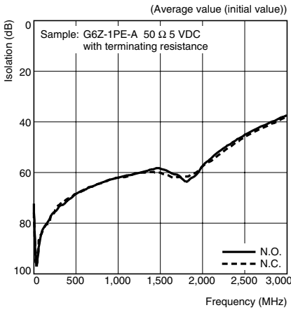
High-frequency Characteristics at 50 Ω (Isolation) (See notes 1 and 2.)
