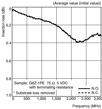
High-frequency Characteristics at 75 Ω (Insertion Loss) (See notes 1 and 2.)
